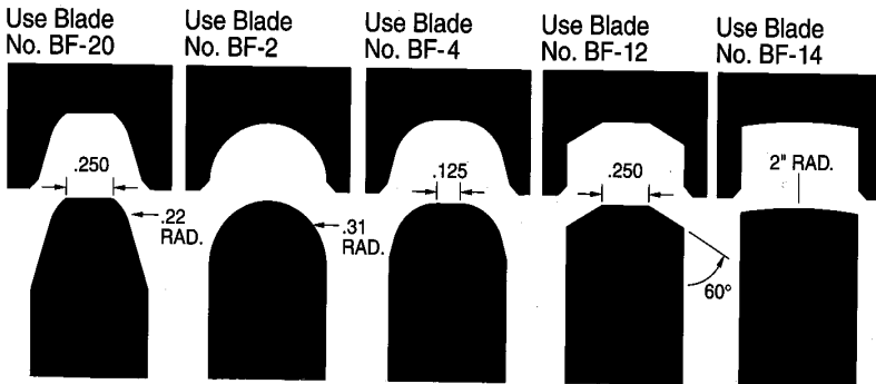
Solid Style Cutters, 1 Piece For #4 & #5RW Electrodes
