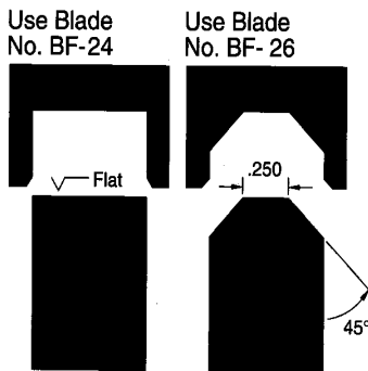
Solid Style Cutters, 1 Piece For #4 & #5RW Electrodes
