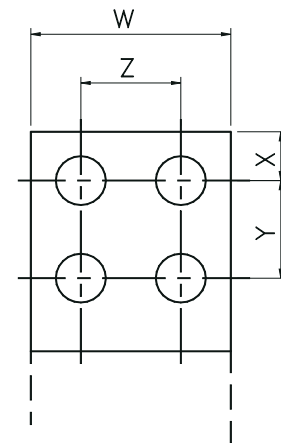
HOLE PATTERN "D"
