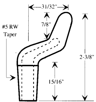
RW-1190 Cold Formed Tip
