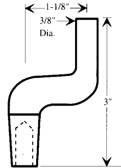
SPB-553-1 / SPB-553-2 (RW-1137 / RW-1138) #4 RW / #5 RW Cold Formed
